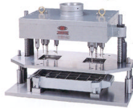
Fix, Guide Bush Plate
