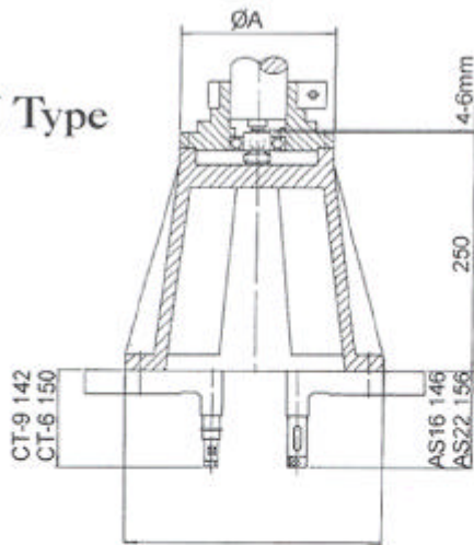
Fix, Adjustable Adapter
